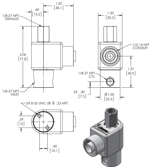
SERIES 50 SLLW MODEL SLLW53 3WNC PIPED EXHAUST LOW WATT
