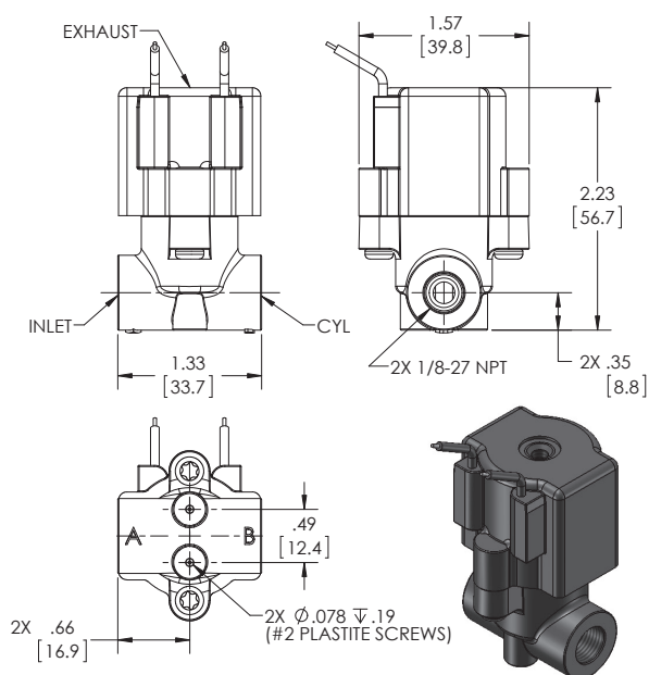
SERIES 40 MODEL 43 (NO BRACKET) 3WNC EXHAUST TO ATMOSPHERE MOLDED WITH LEADS
