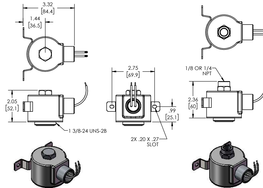
CONDUIT HOUSING WITH MOUNTING BRACKET
