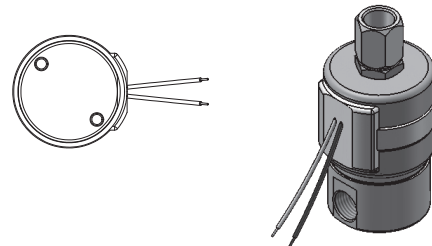
SERIES 20 MODEL 26 3-WAY MULTI-PURPOSE MAGNETIC LATCHING COIL WITH LEADS
