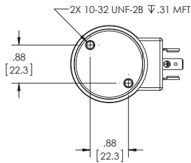
SERIES 20 MODEL 26 3-WAY MULTI-PURPOSE MAGNETIC LATCHING DIN COIL
